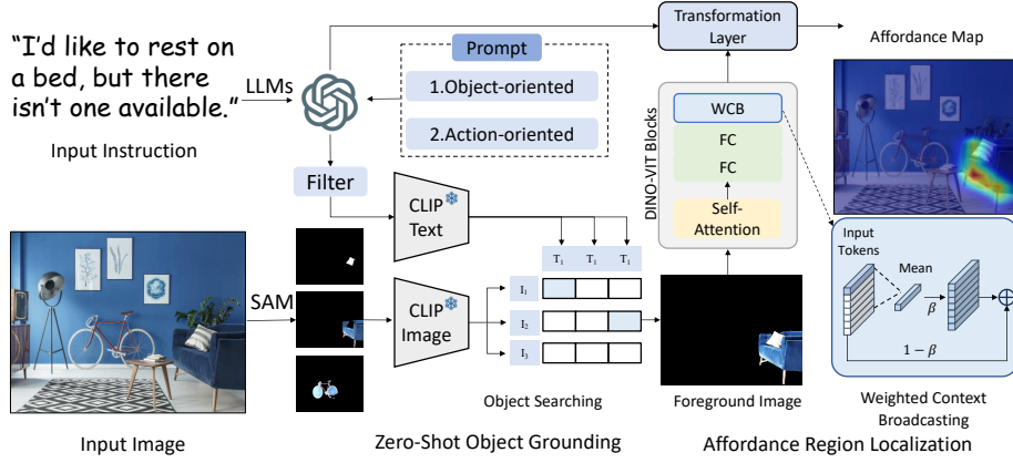
Fig. 5: Framework of WorldAfford. We first derive affordance knowledge from LLMs with the proposed affordance reasoning chain-of-thought. Subsequently, we utilize SAM and CLIP for zero-shot object grounding. Moreover, we design a WCB module and integrate it into the affordance region localization module to localize the affordance regions of multiple objects.
