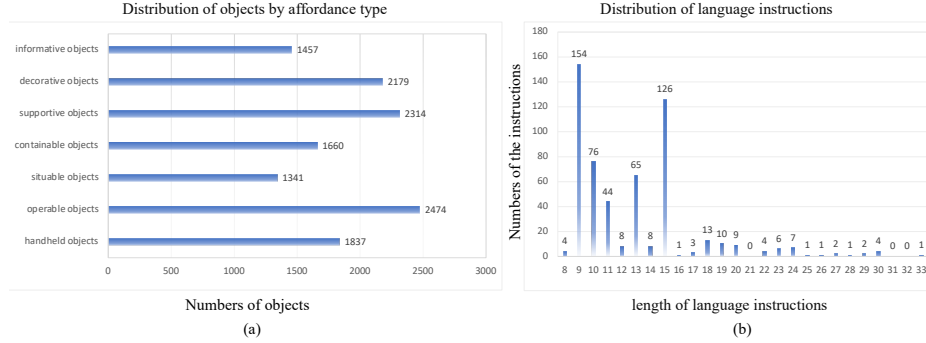
Fig. 3: Statistics of objects and instructions in WorldAfford. (a) Distribution of objects by affordance type. (b) Distribution of language instructions
