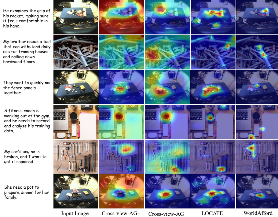
Fig. 8: Visual comparison on the LLMaFF dataset. We manually assign labels to other methods since they cannot adopt the textual input. The labels, "swing", "carry", "catch", "pick up", "catch", and "carry" correspond to the first through sixth rows respectively. The previous approaches cannot predict the affordance regions based on the textual instructions, whereas our method successfully identifies the affordance regions corresponding to natural language instructions and performs outstandingly in the complex environments.
