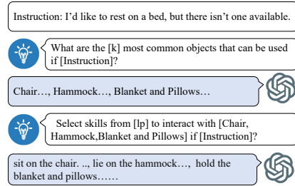
Fig. 6: The affordance reasoning Chain-of-Thought prompting.
