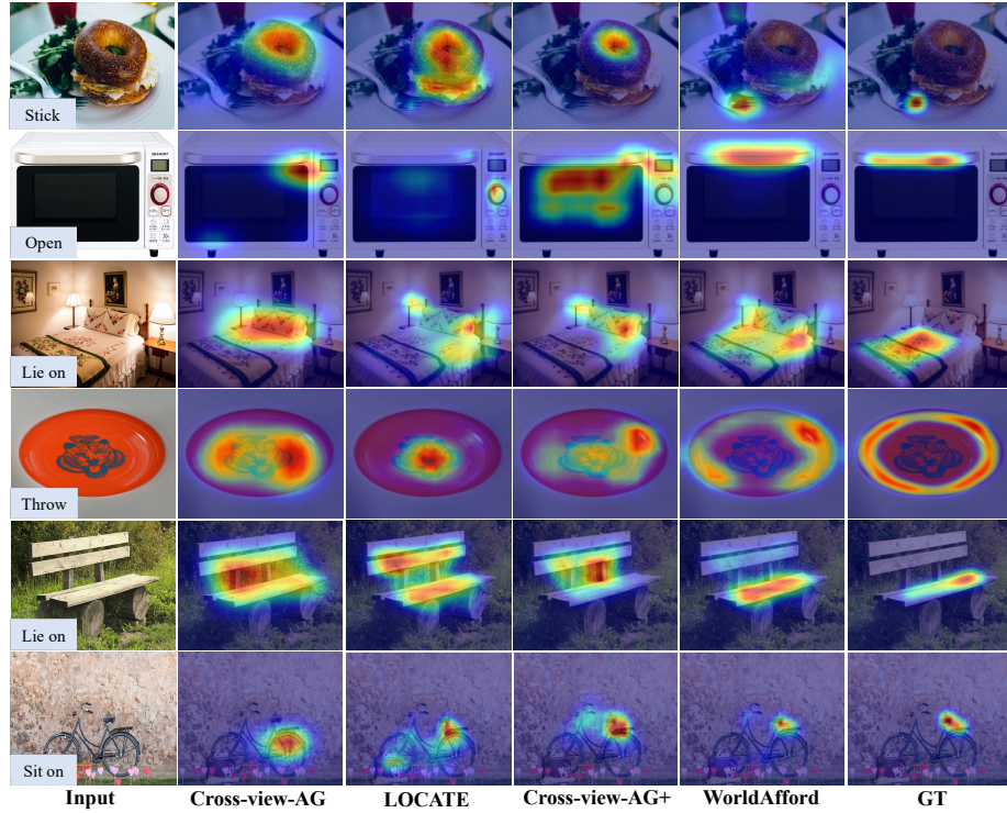
Fig. 7: Visual comparison on the AGD20K dataset. Compared to previous methods, our method can infer more precise affordance maps.
